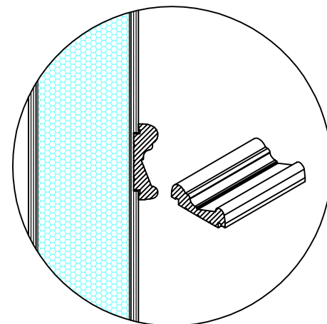
Section drawing: 1-1 Scale 1:3 QW-DBM1 (profile).
