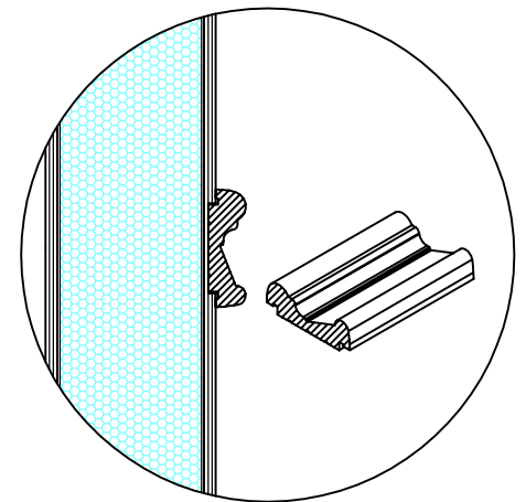
Section drawing: 1-1 Scale 1:3 QW-DBM1 (profile).
